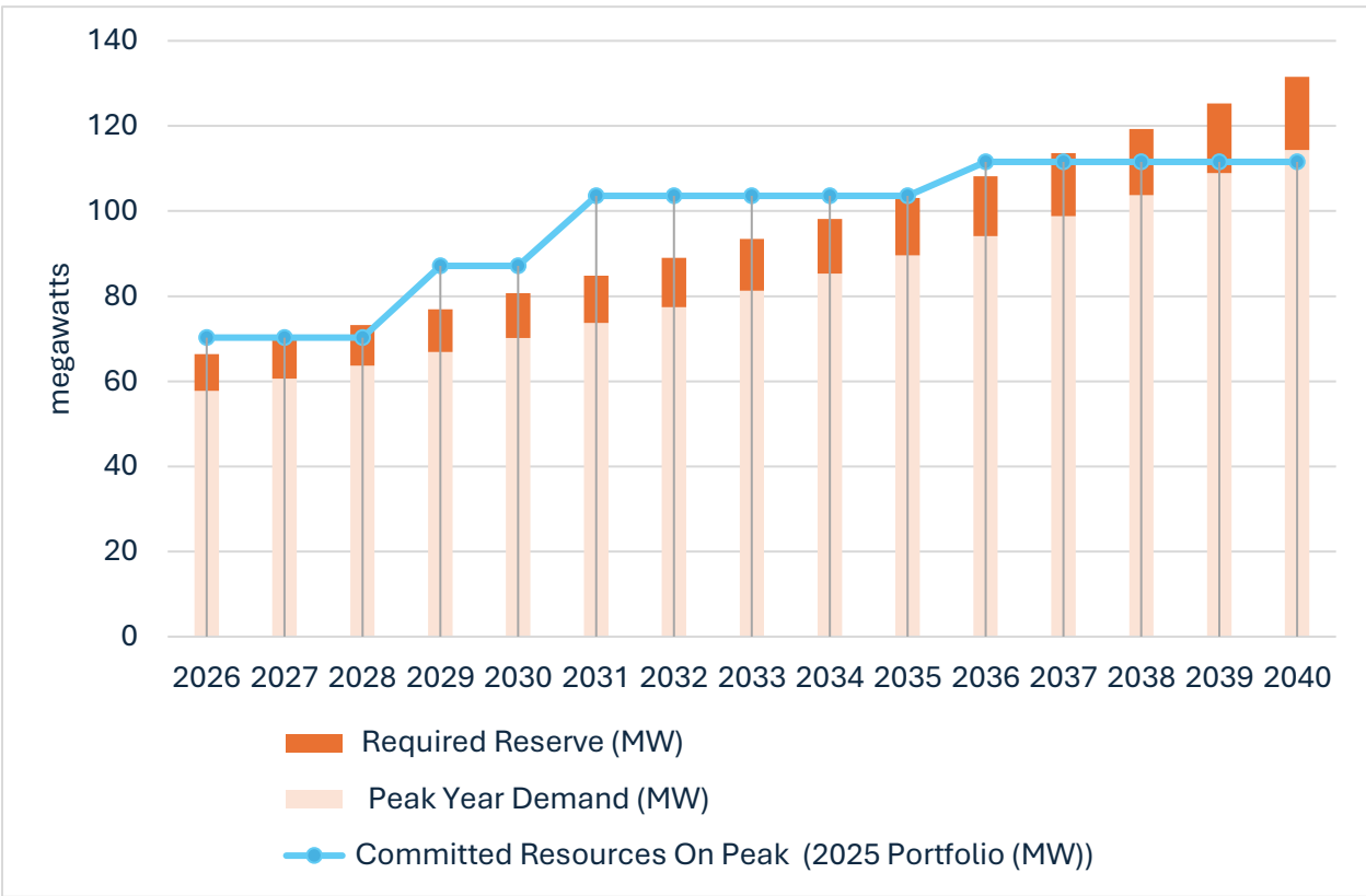
CHART 8-1: PREFERRED PORTFOLIO PROJECTED CAPACITY SURPLUS/DEFICIT
