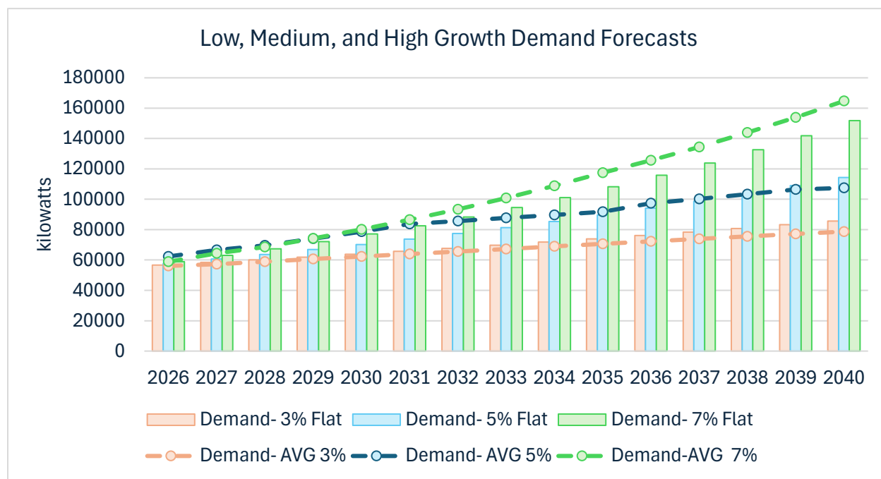
CHART 5-2: FORECAST OF ANNUAL SYSTEM PEAK (2026-2040)
