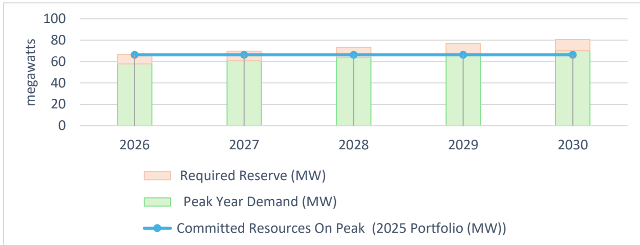
CHART 7-1: CAPACITY AND ENERGY BALANCE- CURRENT PORTFOLIO WITHOUT NEW RESOURCES
