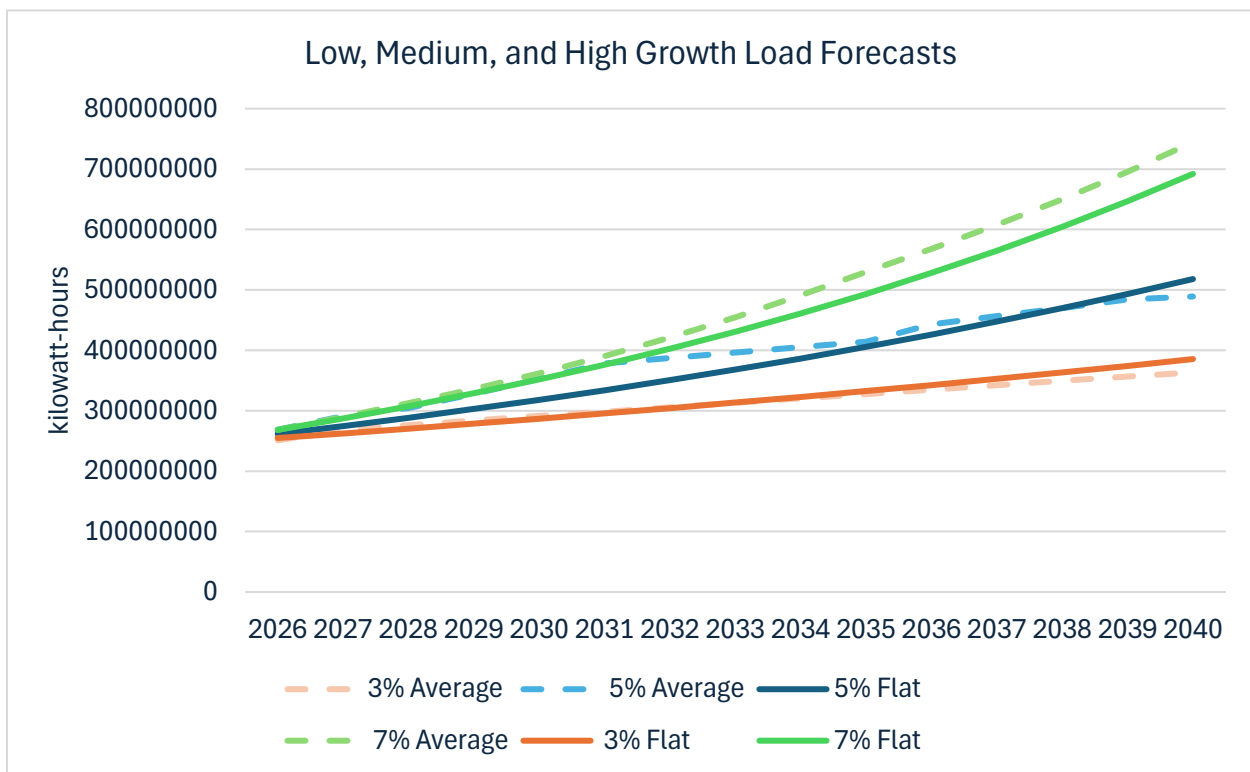
CHART 5-1: FORECAST OF ANNUAL SYSTEM LOAD (2026–2040)
