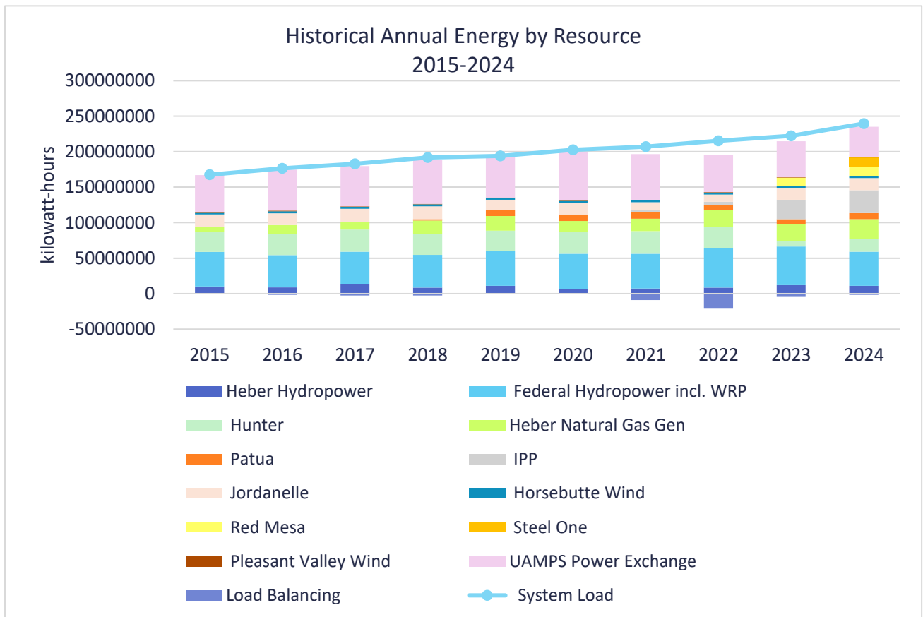
CHART 6-1: HISTORICAL ANNUAL ENERGY BY RESOURCE (2015–2024)
